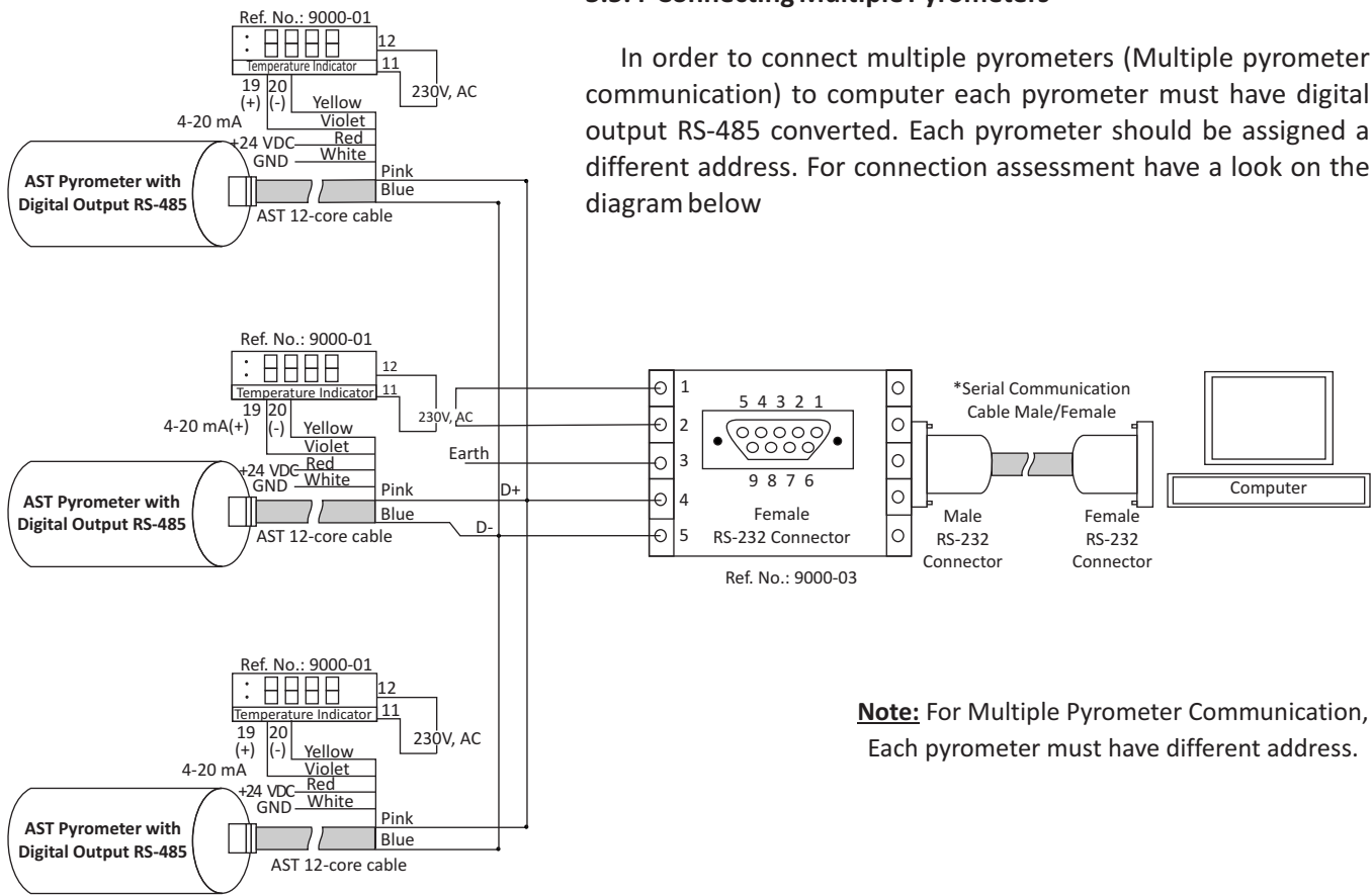
Fig. 20 Multi-Pyrometer Connection
