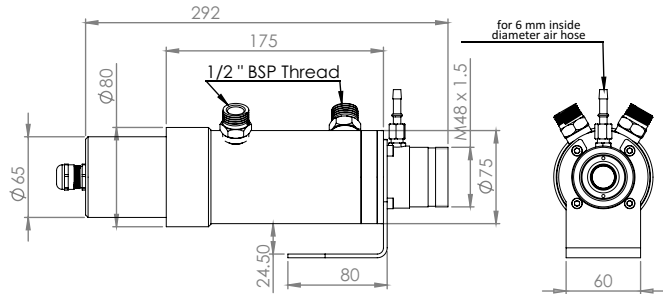
Water Cooling Jacket with Adjustable Flange PL (Reference no: 8000-08)
