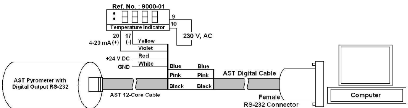
RS-232 Connection
